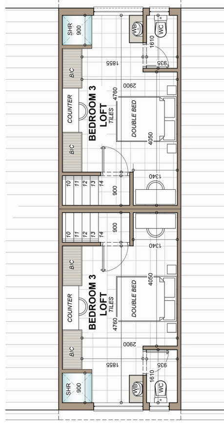
LOFT FLOOR PLAN NOT TO SCALE
